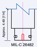
MIL-C 26482 Dimensions in inches [mm]
